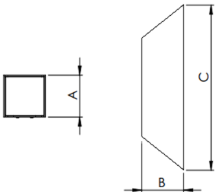
A = 300mm | B = 76mm | C = 76mm
