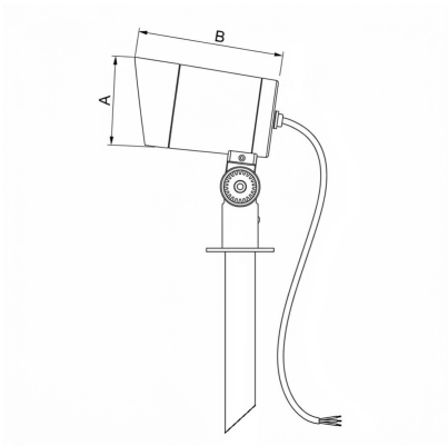
A = 180mm | B = Ø75mm
